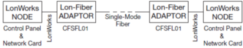
Fiber Optic Point to Point Link
