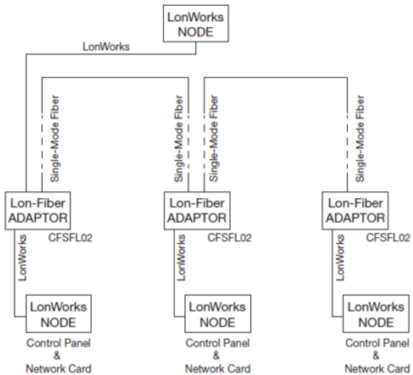
Fiber Optic Star Topology Link
