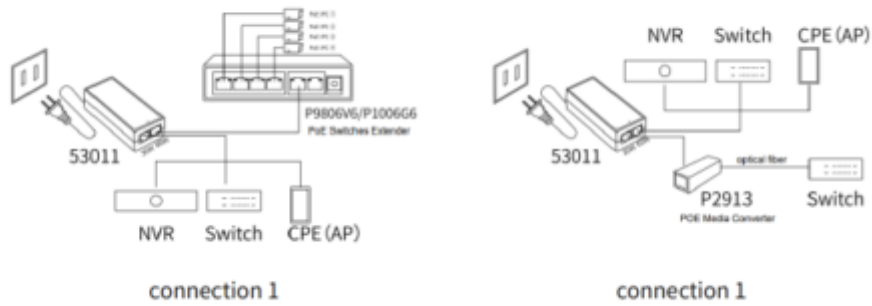
PoE Power adapter connection diagram
